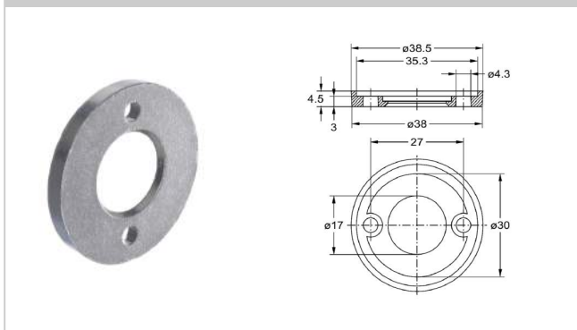
3005 Levelling piece
