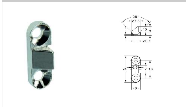
2704 Strike plate
