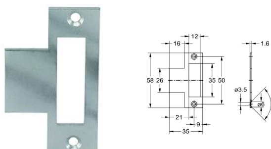
2527 Strike plate
