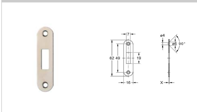
2584 Strike plate
