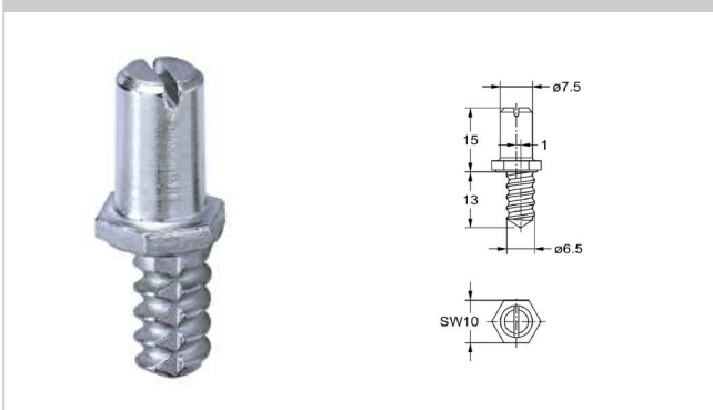
2533 Joint bolt
