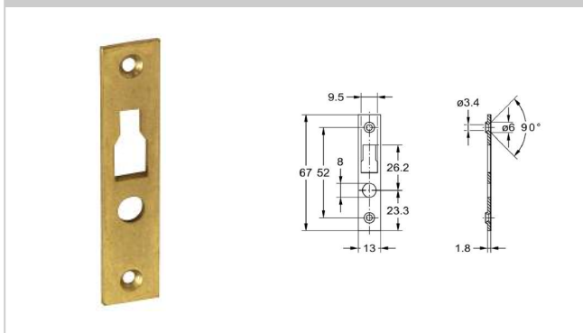
2514 Strike plate
