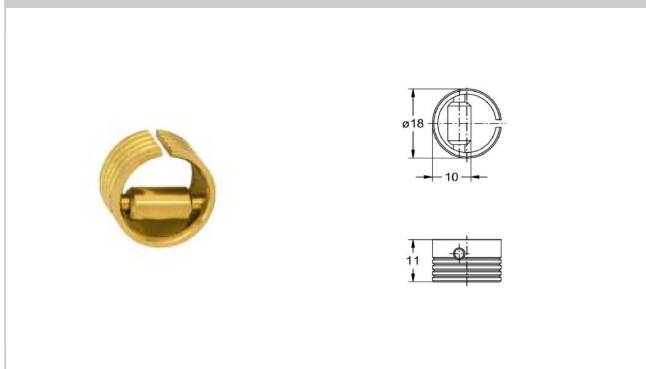
2511 Spring-loaded strike plate
