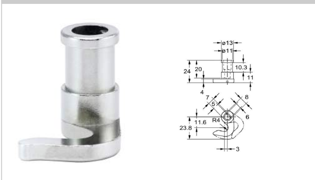
2415 Hook bolts
