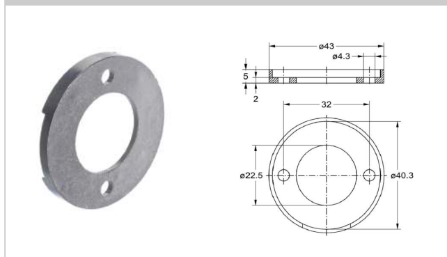
3006 Levelling piece
