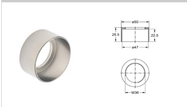
2617 Tube nut
