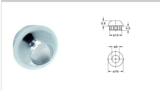
2703 Locking case
