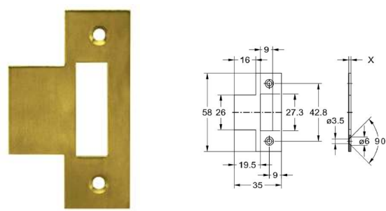
2523 Strike plate
