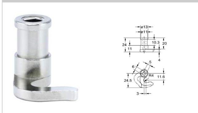
2423 Hook bolts
