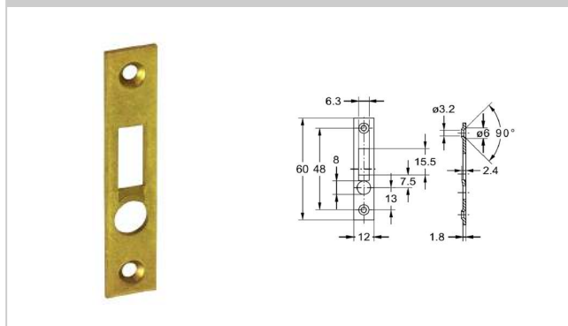
2515 Strike plate
