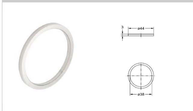
2618 Spacer washer
