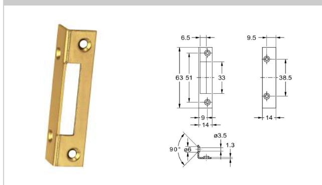
2596 Strike plate
