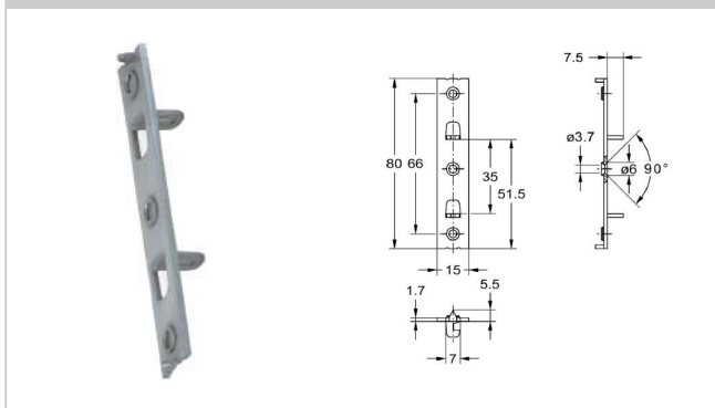
2591 Strike plate
