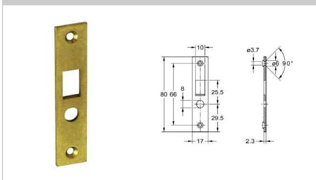
2516 Strike plate
