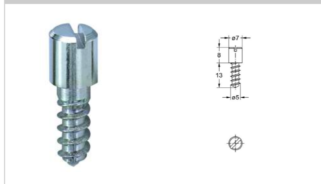
2534 Joint bolt
