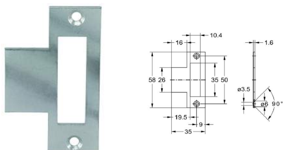
2522 Strike plate
