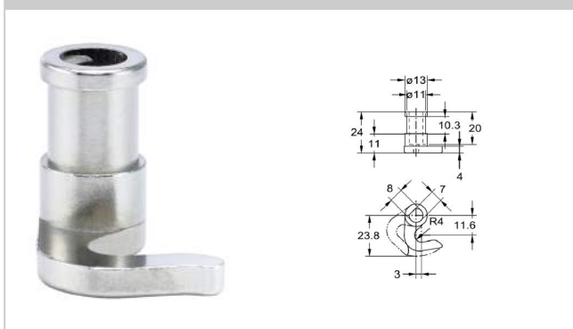
2425 Hook bolts
