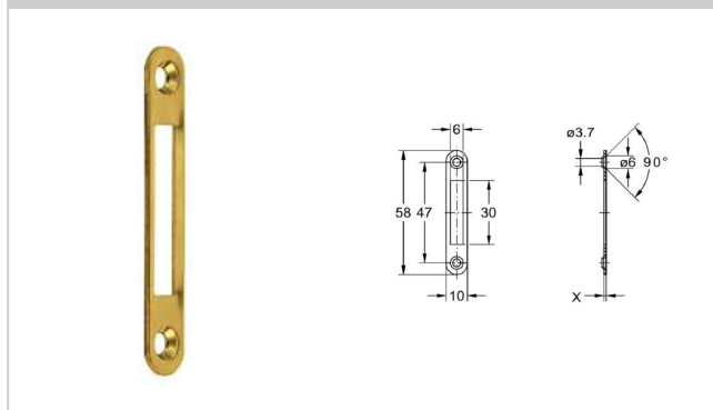
2585 Strike plate
