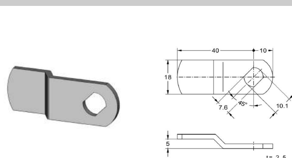
2642.402 Lever
