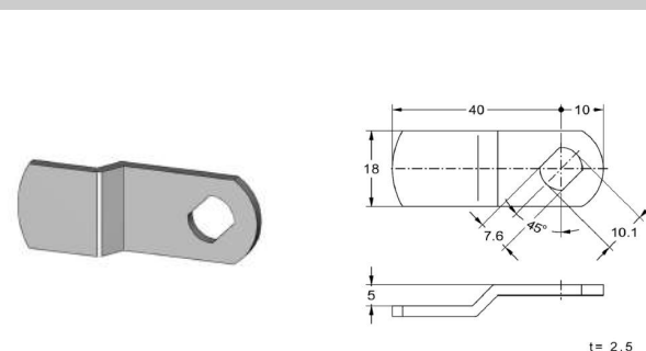
2641.402 Lever
