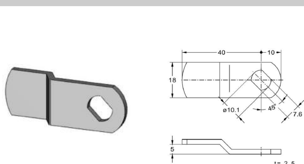
2642.401 Lever
