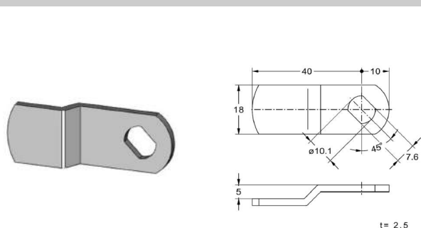
2641.401 Lever
